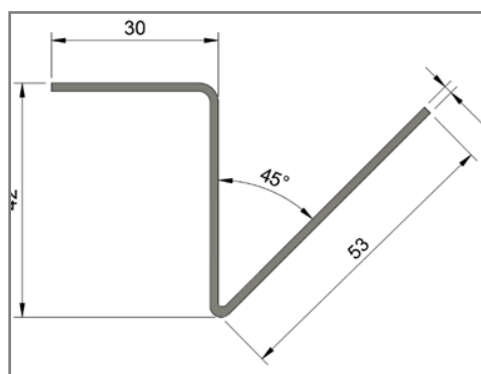
("ill. 3" - Dimensioner VTO rende—PVC)
